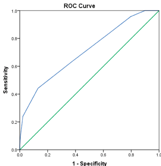
Fig. 2. ROC curve predicting the DJSS.
