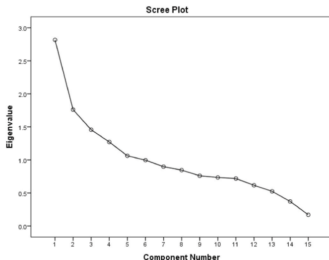
Fig. 1. Scree plot for the 15 determinants of DJSS.
